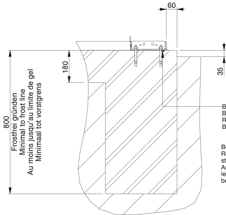
SECTION E-E SCALE 1:10
