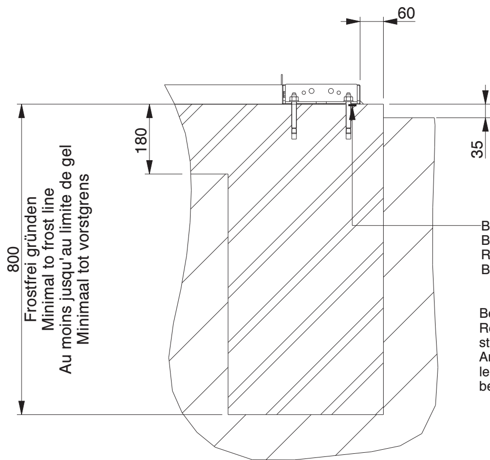
SECTION E-E SCALE 1:10
