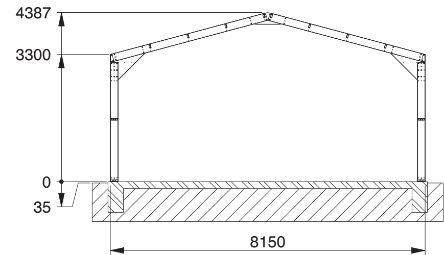
SECTION E-E
