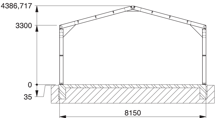
SECTION E-E
