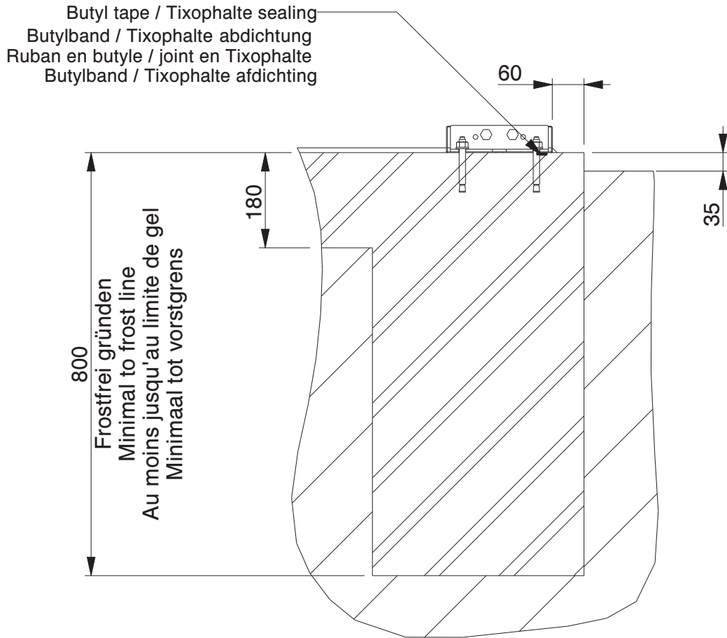
SECTION E-E SCALE 1:10
