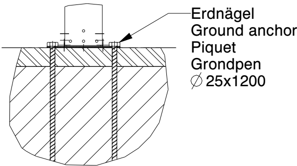
SECTION C-C SCALE 1:20
