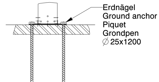
SECTION C-C SCALE 1:20
